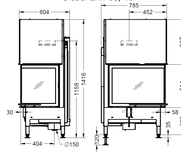
Global 2Rh 68/48
